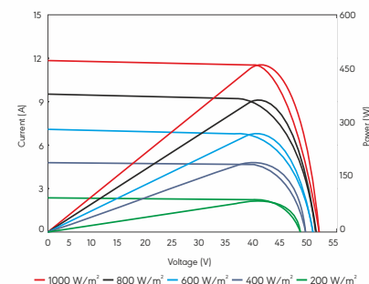
I-V Curves of PV Module (for Ref)
